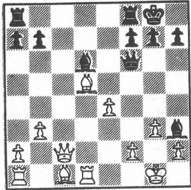
378 After 17 Rd1
